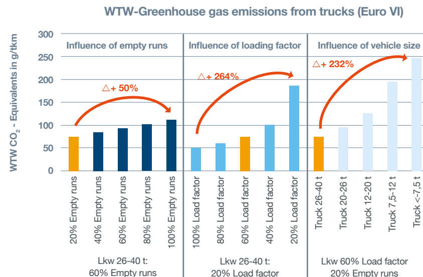
Figure 3 Impact of empty trip share, filling rate and vehicle size on emissions 26
