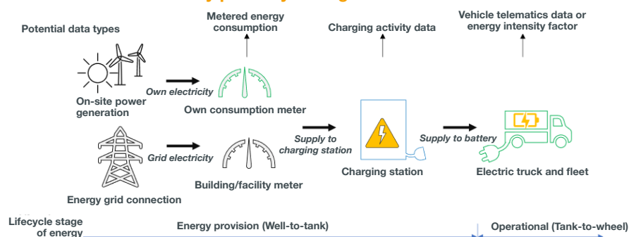
Figure 2 Illustration of electricity pathway from grid meter to vehicle and the various data
